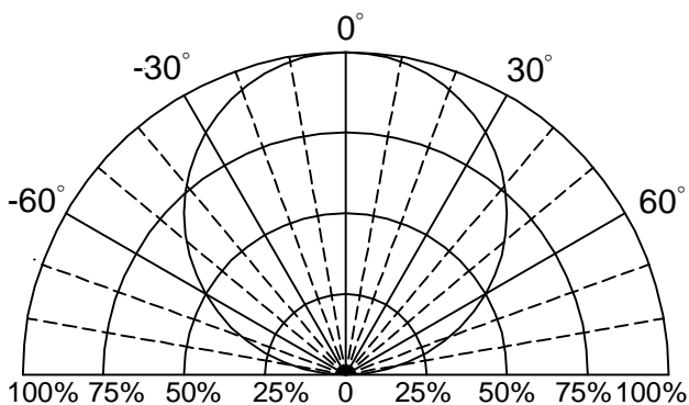
Fig.5 Directivity Radiation
