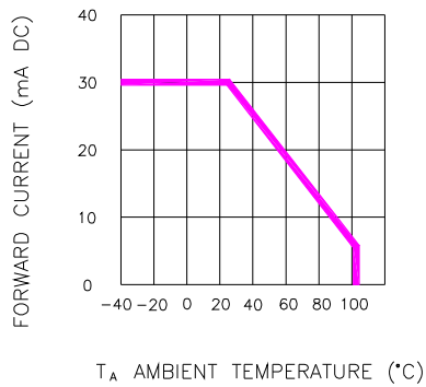
Fig.5 FORWARD CURRENT VS. AMBIENT TEMPERATURE
