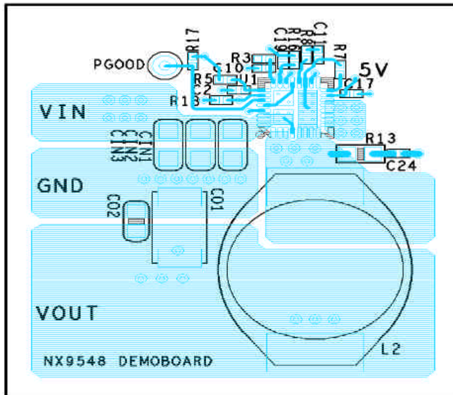
Figure 15 Top layer
