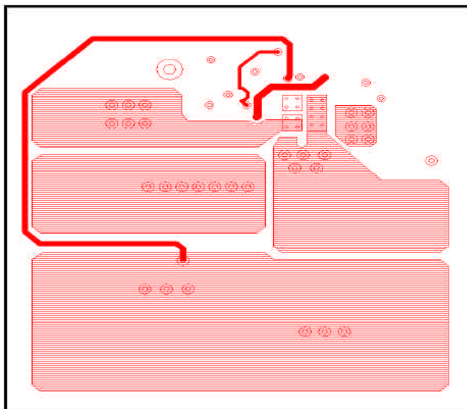
Figure 18 Bottom layer
