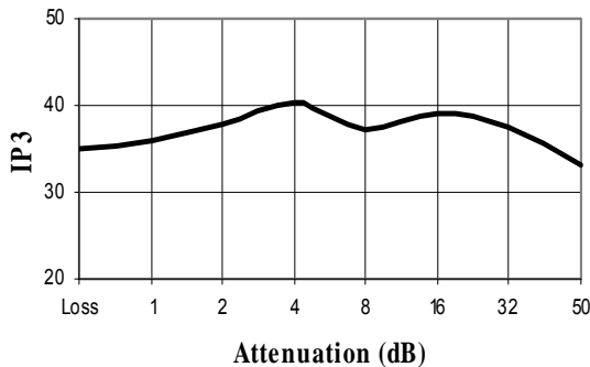
Maximum IP3 over Temperature Range and Attenuation @ 50 MHz
