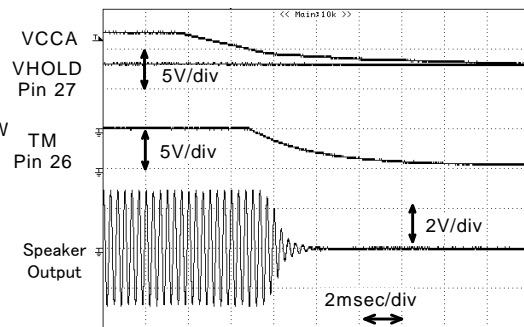
Fig. 16 Wave form on Instantaneous Power Interruption (2msec / div)
