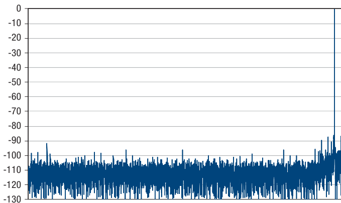
FFT 16384 points Fs: 4.85 MHz Fs: 10MHz Range pin voltage: 1V
