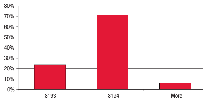
Cross-talk Grounded Input Histogram Test Channel tied to GND – Other 3 Channels with 2.45 MHz FS Input Signal
