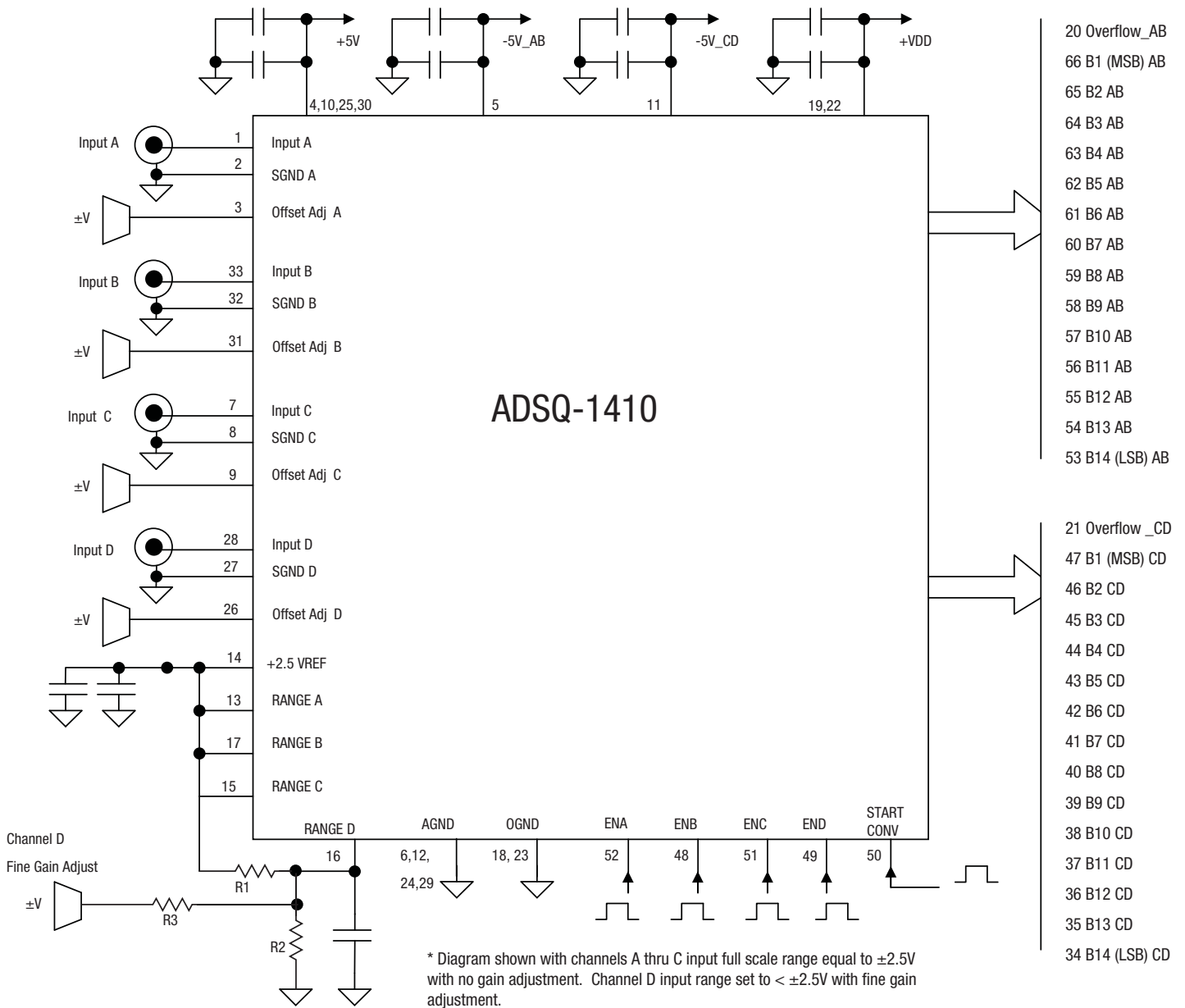
Connection Diagram
