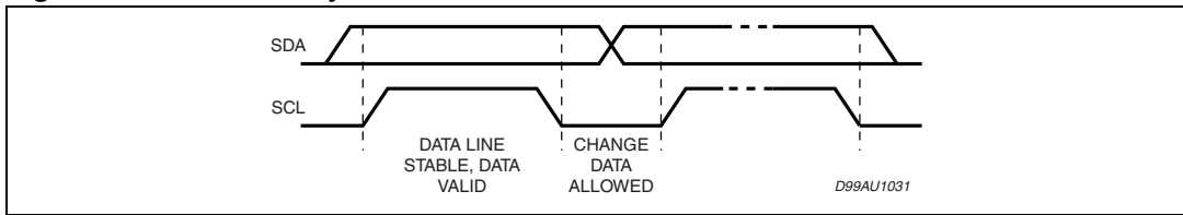
Figure 4. Timing diagram of I 2 C BUS
