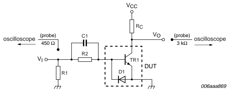
I_C = 0.05\text{ A}; I_B = 2.5\text{ mA}; R_1 = 50\ \Omega; R_2 = 3\text{ k}\Omega; R_C = 180\ \Omega; C_1 = 1\text{ nF}
