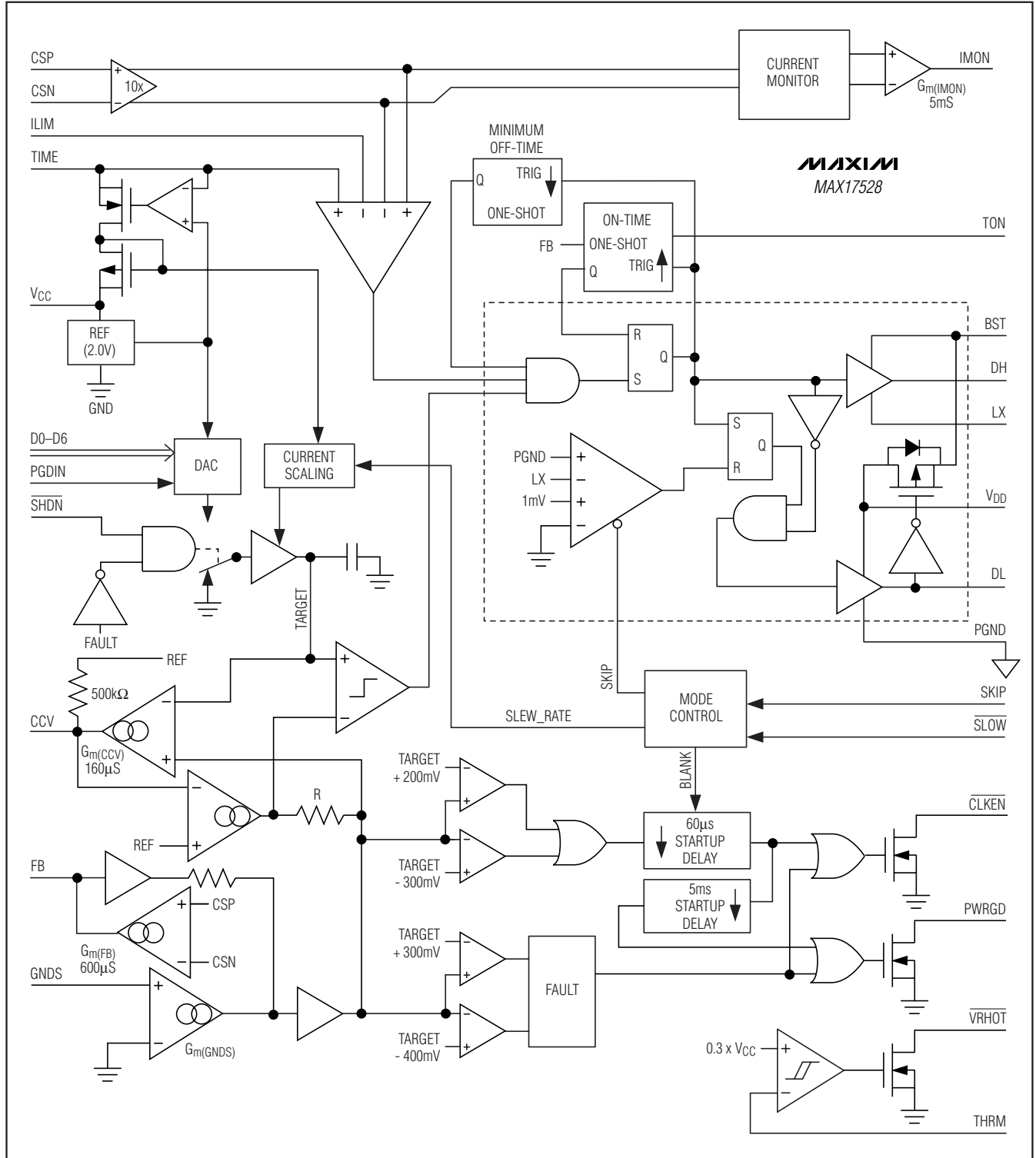
Figure 3. Functional Diagram
