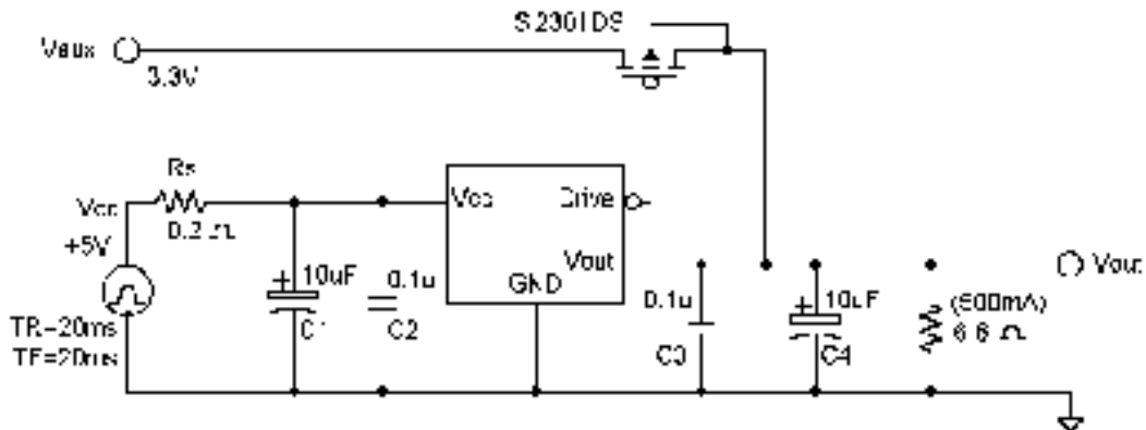
Figure 6. Transient Characteristics Test Set-up
