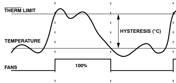
Figure 29. THERM Temperature Limit Operation
