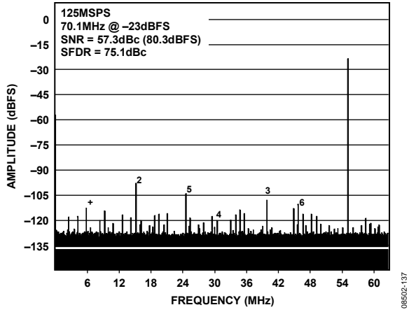
Figure 37. AD9265-125 Single-Tone FFT with f_{IN} = 70.1 MHz @ -23 dBFS with Dither Disabled, 1M Sample
