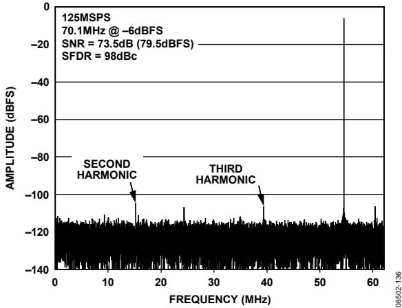
Figure 36. AD9265-125 Single-Tone FFT with f_{IN} = 70.1 MHz @ -6 dBFS with Dither Enabled
