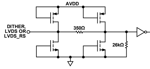
Figure 63. Equivalent DITHER, LVDS, and LVDS_RS Input Circuit
