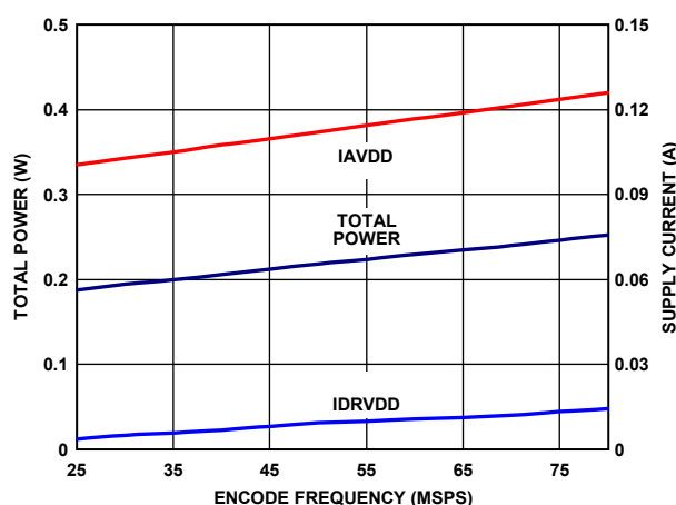
Figure 83. AD9265-80 Power and Current vs. Sample Rate
