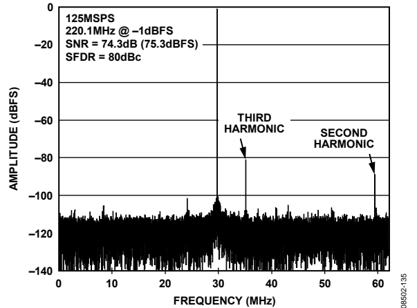
Figure 35. AD9265-125 Single-Tone FFT with f_{IN} = 220.1 MHz
