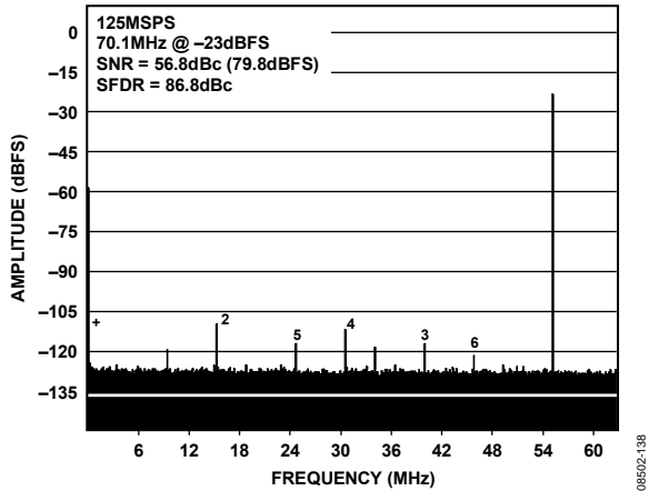
Figure 38. AD9265-125 Single-Tone FFT with f_{IN} = 70.1 MHz @ -23 dBFS with Dither Enabled, 1M Sample
