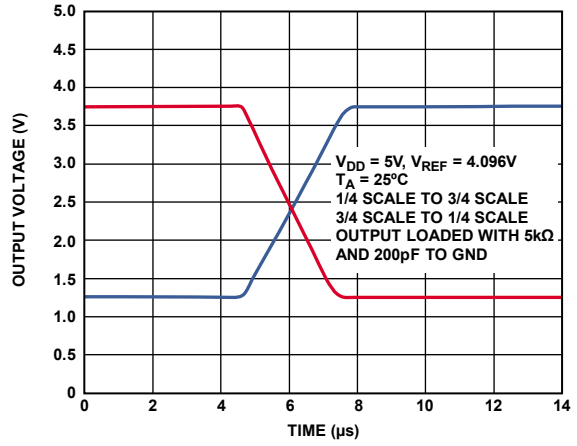
Figure 21. Settling Time and Typical Output Slew Rate
