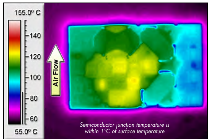
Figure 6: Thermal plot of converter at 6.7 amp load current with 55°C air flowing at the rate of 200 LFM. Air is flowing across the converter sideways from pin 3 to pin 1 (24V input).
