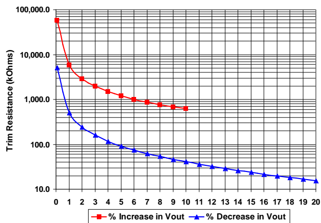
Figure C: Trim Graph for 8.0Vout module
