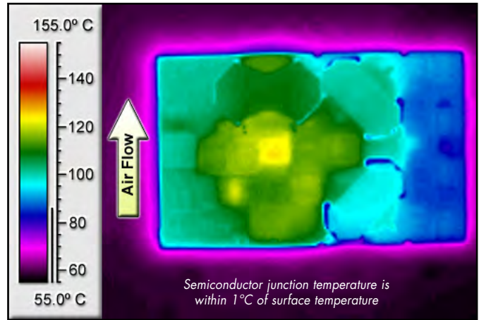
Figure 8: Thermal plot of converter at 6.2 amp load current with 55°C air flowing at the rate of 200 LFM. Air is flowing across the converter sideways from pin 3 to pin 1 (48V input).
