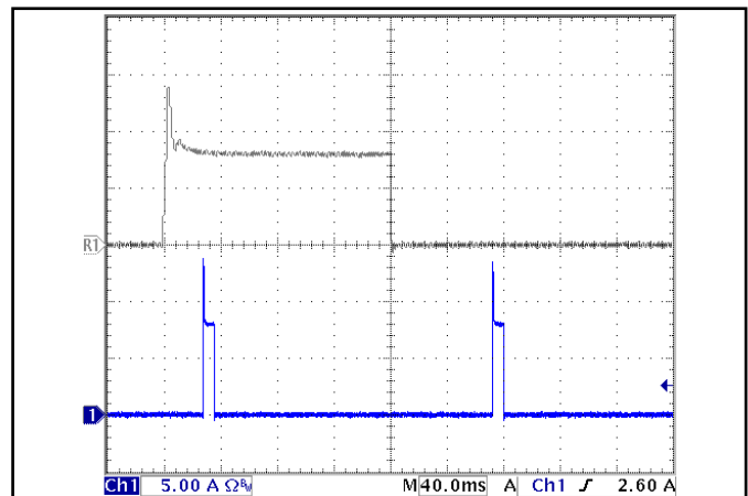
Figure 22: Load current (5 A/div) as a function of time when the converter attempts to turn on into a 10\ \text{m}\Omega short circuit. Top trace (40 ms/div) is an expansion of the on-time portion of the bottom trace.
