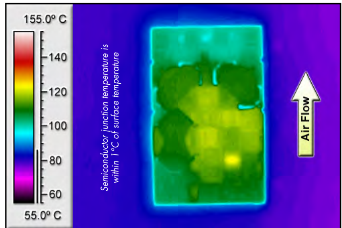
Figure 10: Thermal plot of converter at 6.7 amp load current with 85°C air flowing at the rate of 200 LFM. Air is flowing across the converter from input to output (24V input).
