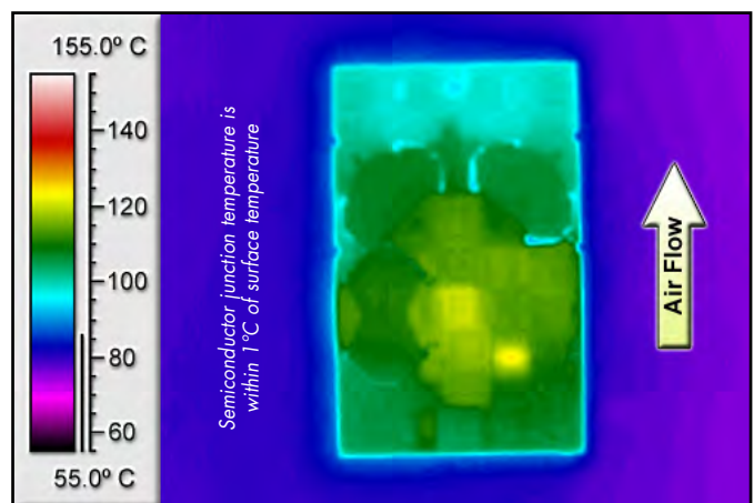
Figure 12: Thermal plot of converter at 6.2 amp load current with 85°C air flowing at the rate of 200 LFM. Air is flowing across the converter from input to output (48V input).
