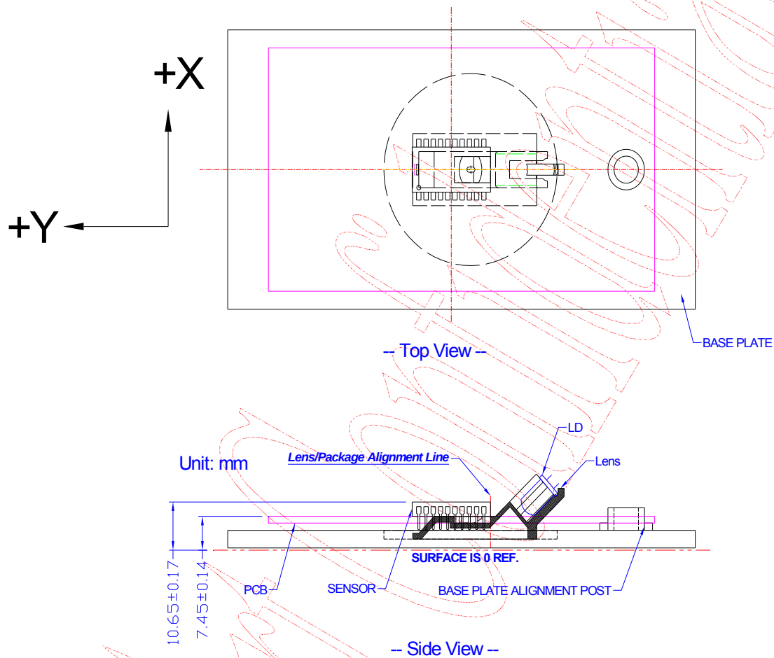
Figure 20. 2D Assembly
