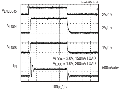
LD04 AND LD05 STARTUP AND SHUTDOWN WAVEFORM
