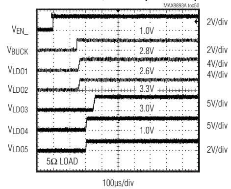
POWER-UP SEQUENCING (MAX8893A)
