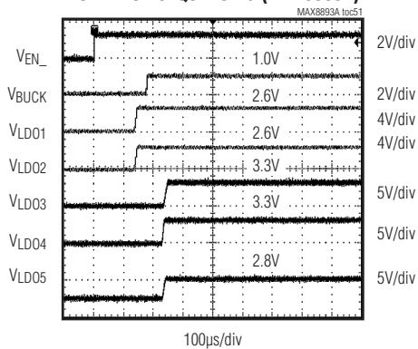
POWER-UP SEQUENCING (MAX8893B)
