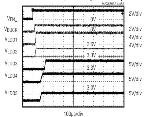
POWER-UP SEQUENCING (MAX8893C)
