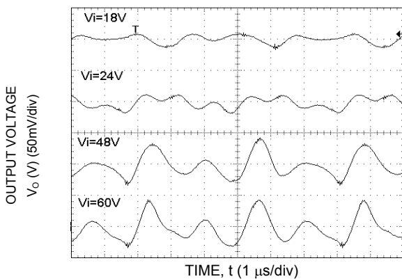
Figure 3. Typical Output Ripple and Noise at V_o = 3.3\text{V} and I_o = 20\text{A} .
