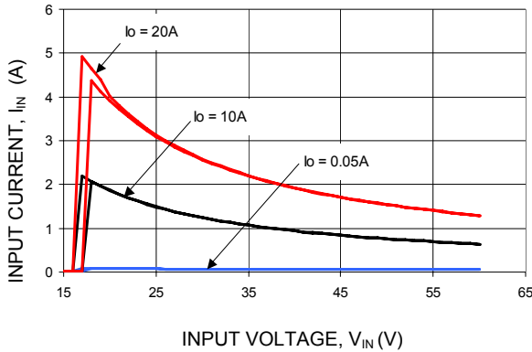
Figure 1. Typical Input characteristics at room temperature ( V_o = 3.3\text{V} ).
