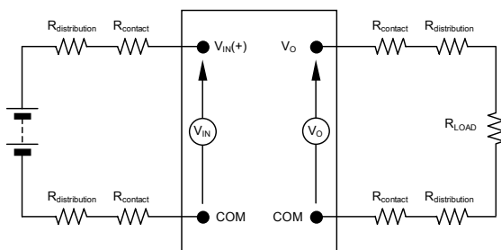
Figure 18. Output Ripple and Noise Test Setup.
