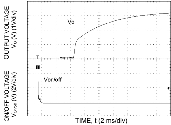
Figure 4. Typical Start-Up Characteristics from Remote ON/OFF ( V_o = 3.3\text{V} , I_o = 20\text{A} , V_{in} = 48\text{V} ).
