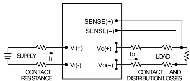
Figure 21. Effective Circuit Configuration for remote sense operation.
