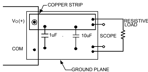
Figure 17. Input Reflected Ripple Current Test Setup.
