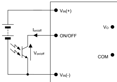
Figure 20. Circuit configuration for using Remote On/Off Implementation.
