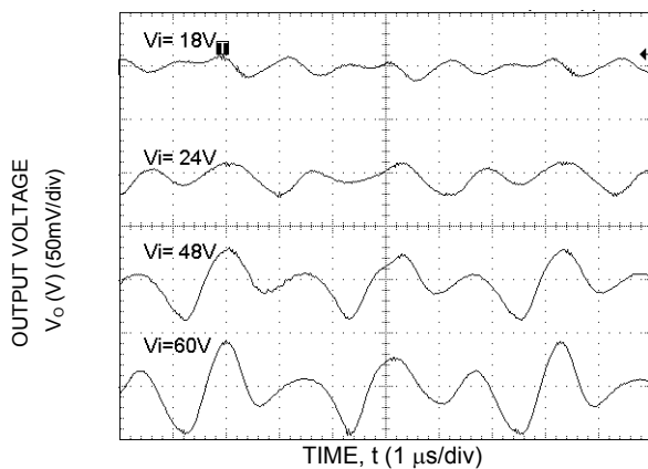
Figure 9. Typical Output Ripple and Noise at V_o = 5\text{V} and I_o = 15\text{A} .
