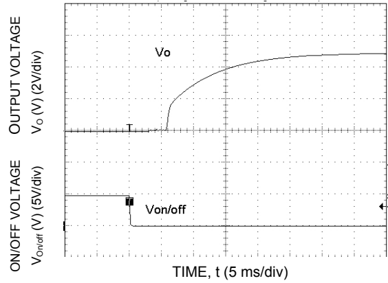
Figure 10. Typical Start-Up Characteristics from Remote ON/OFF ( V_o = 5\text{V} , I_o = 15\text{A} , V_{in} = 48\text{V} )
