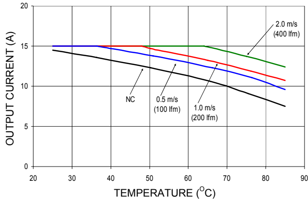
Figure 13. Thermal Derating Curves for the EQD075 module at 24Vin and V_o=5V .
