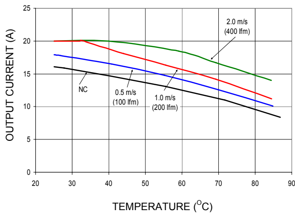
Figure 15. Thermal Derating Curves for the EQD075 module at 24Vin and V_o=3.3V .
