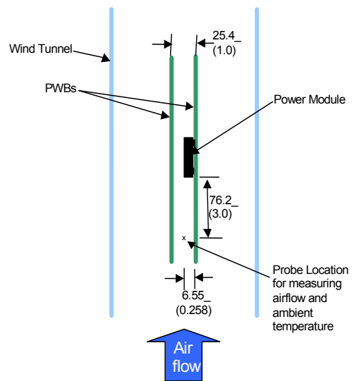
Figure 23. Thermal Test Set up.
