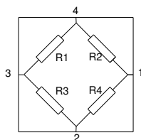
electrical diagram:
