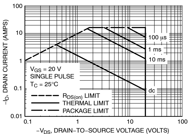
Figure 22. Maximum Rated Forward Biased Safe Operating Area
