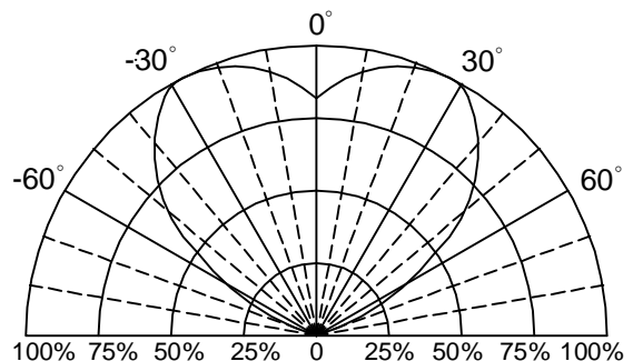
Fig.6 Directivity Radiation
