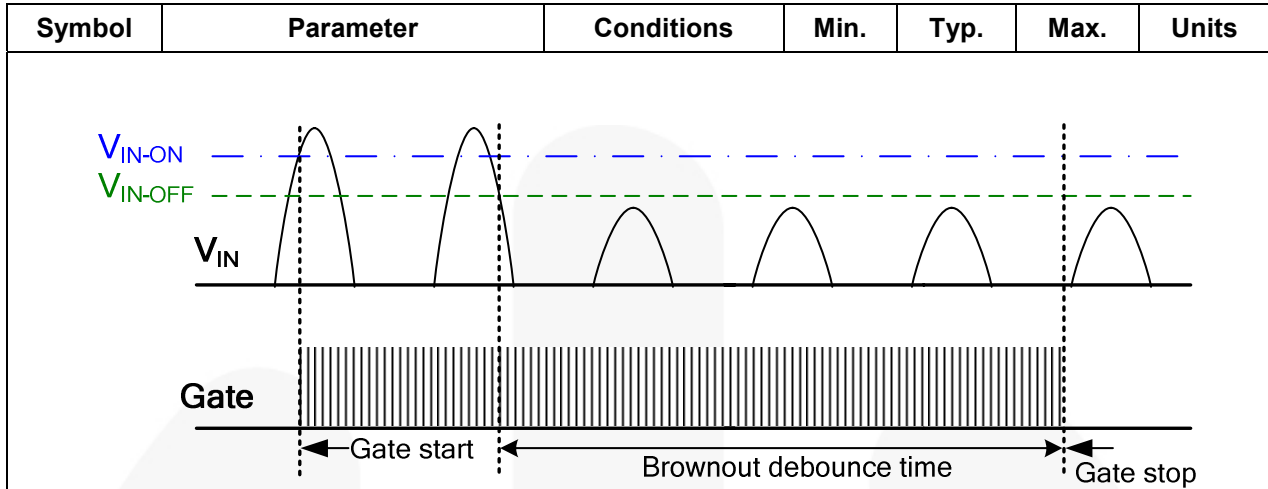
Figure 8. Brownout Behavior
