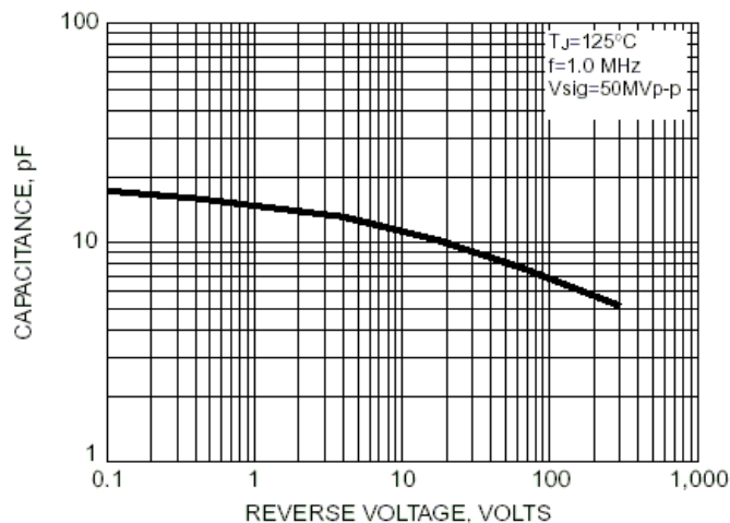
FIG. 6 - TYPICAL JUNCTION CAPACITANCE PER LEG
