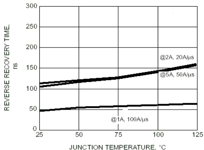
FIG. 5 - REVERSE SWITCHING CHARACTERISTICS PER LEG
