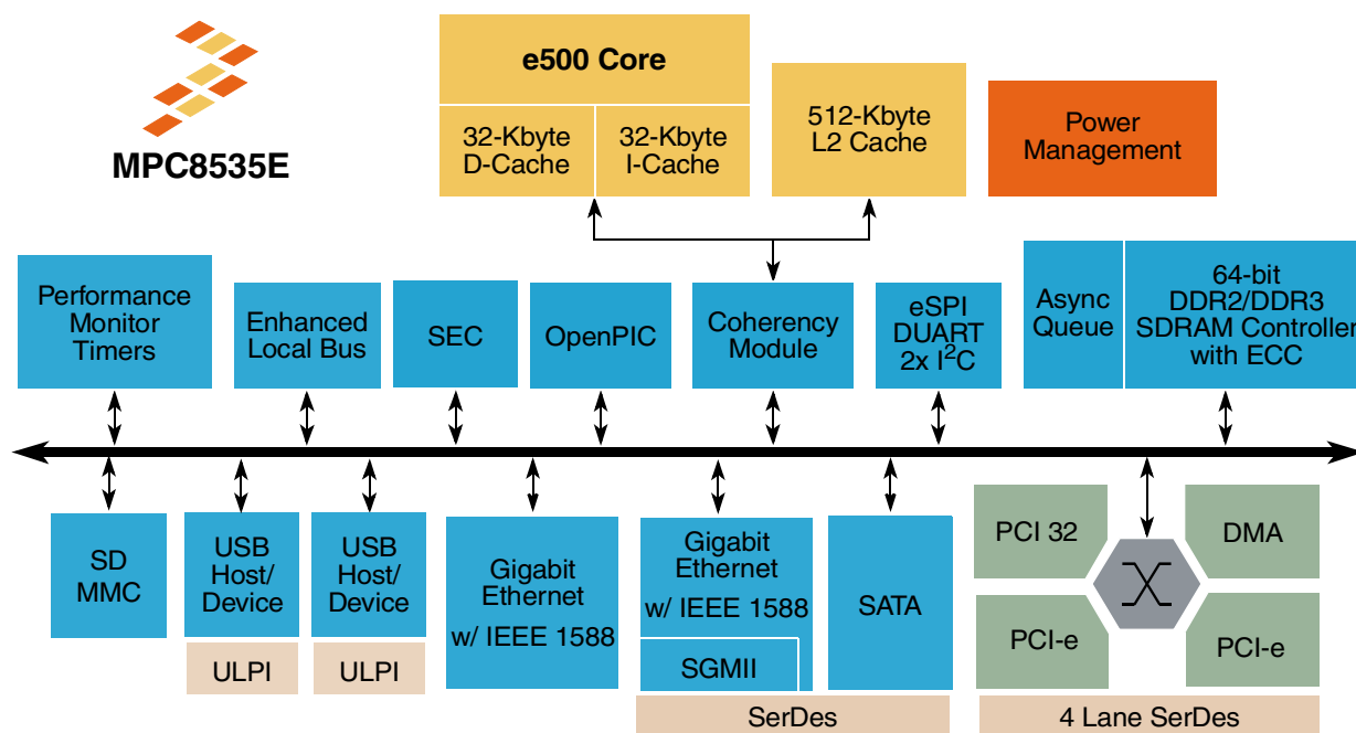
Figure 1. MPC8535E Block Diagram
