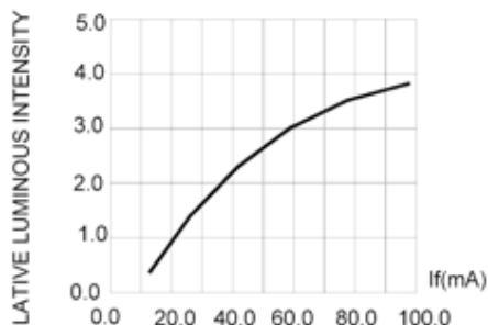
FIG.3 FORWARD CURRENT.
