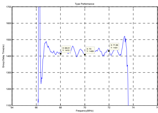
Group Delay Variation(f0±2MHz)
