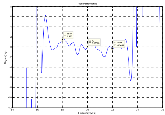
Phase Linearity(f0±2MHz)
