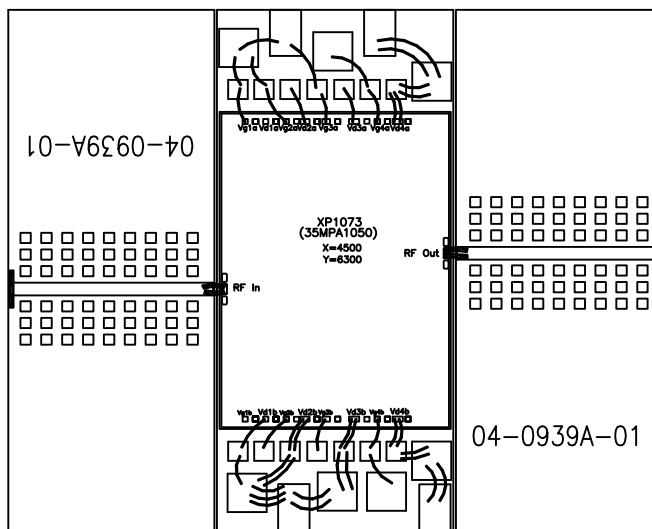
Layout for reference only – It is recommended to bias output stage from both sides.
