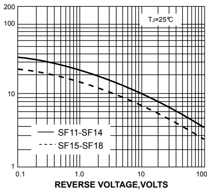
FIG. 5-TYPICAL JUNCTION CAPACITANCE
