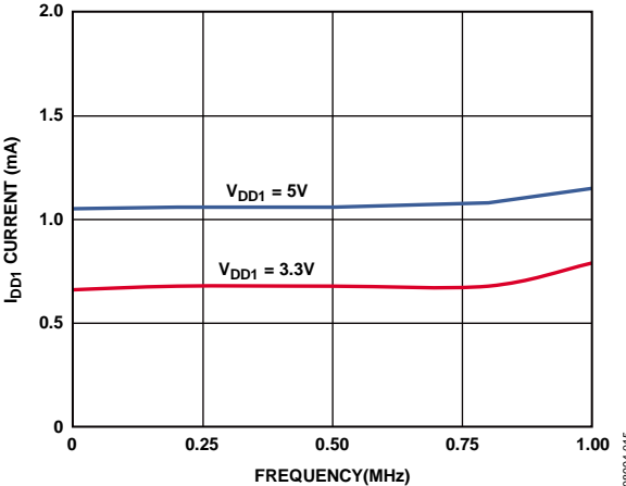
Figure 8. Typical I_{DD1} Supply Current vs. Frequency
