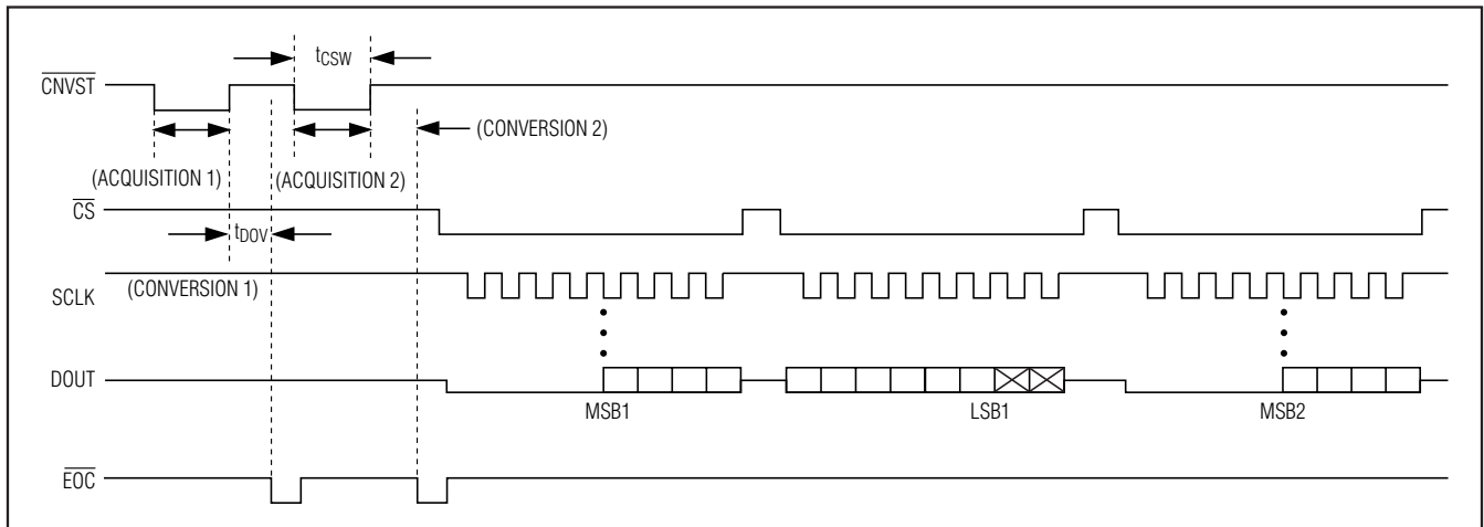
Figure 7. Clock Mode 01—After writing a command byte, request multiple conversions by setting \overline{CNVST} low for each conversion.
