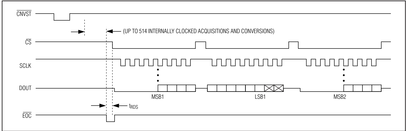
Figure 6. Clock Mode 00—After writing a command byte, set \overline{CNVST} low for at least 40ns to begin a conversion.
