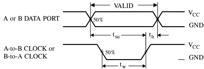
Figure 7. Switching Waveforms
