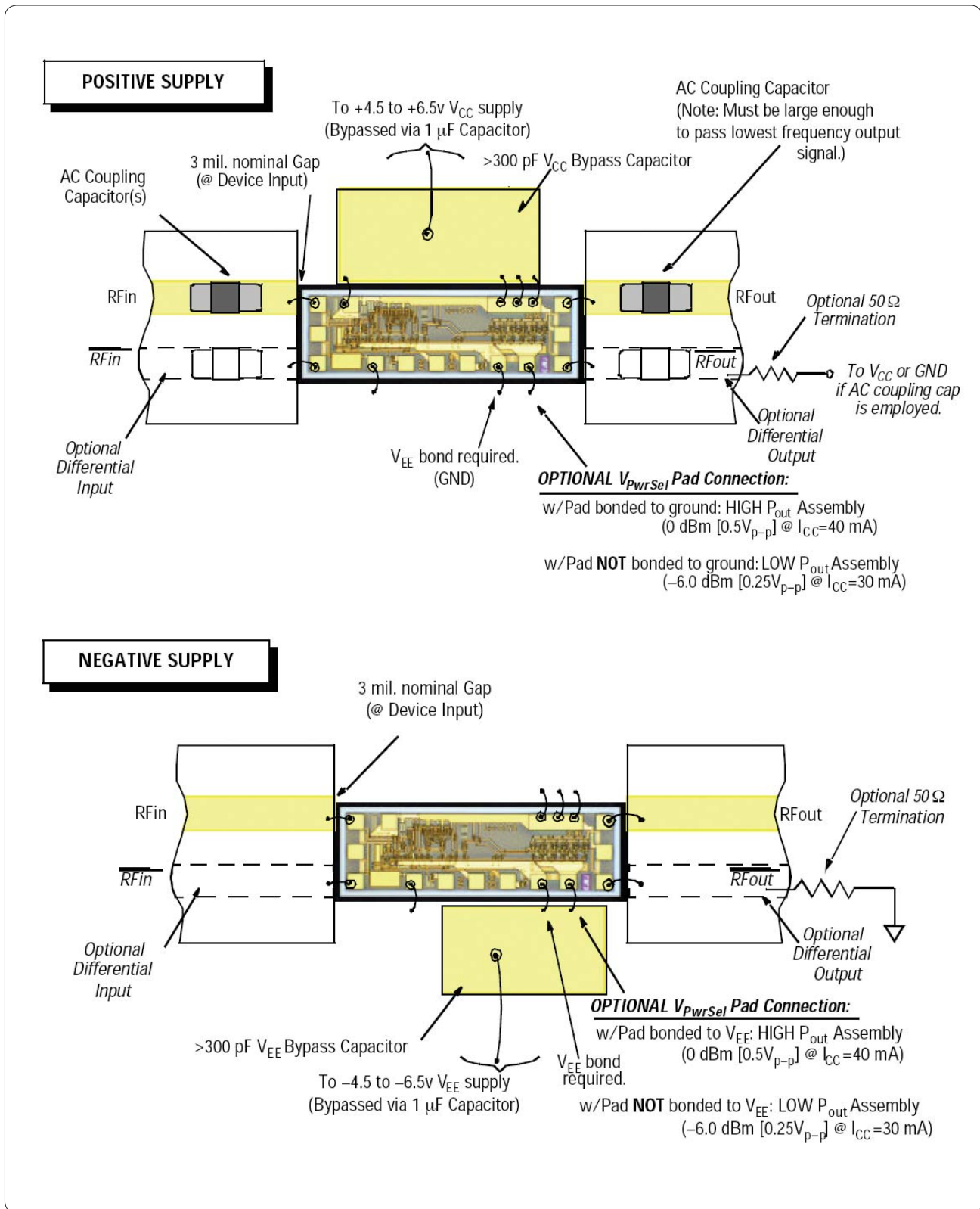
Figure 3. Assembly diagrams
