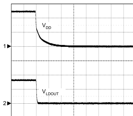
LDO Power Off
