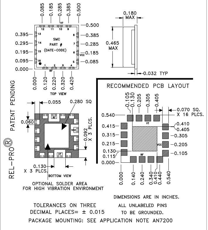
Package # 278LF
