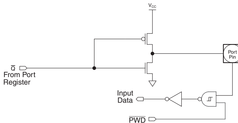
Figure 10-5. Push-pull Output
