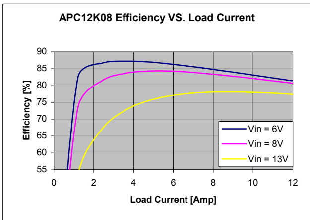
Figure 17. APC12K08 Efficiency Curve.
