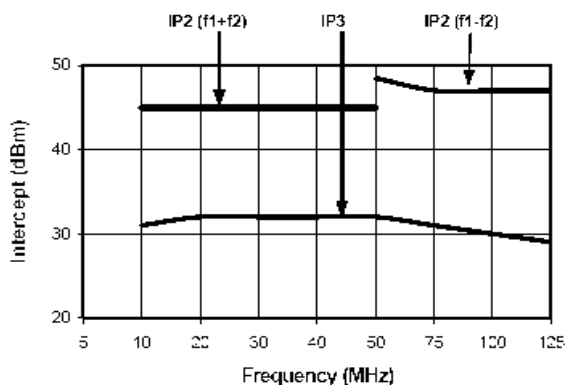
Intermodulation Intercept
