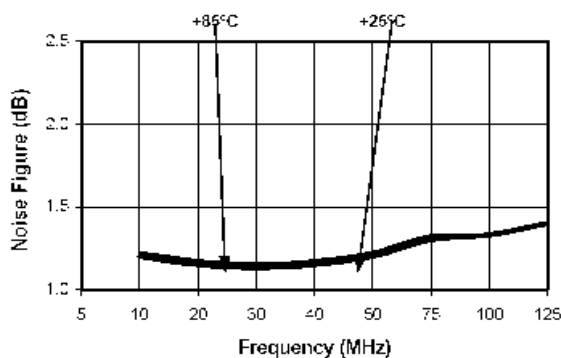
Noise Figure
