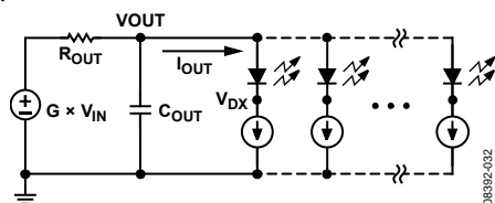
Figure 47. Charge Pump Equivalent Circuit Model
