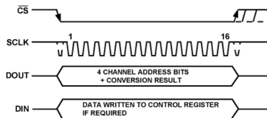
Figure 6. Normal Mode Operation
