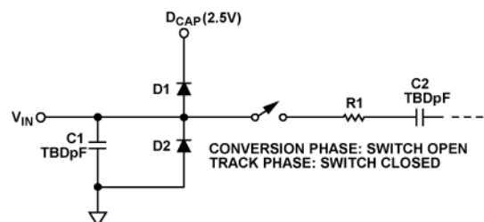
Figure 10. Equivalent Analog Input Circuit
