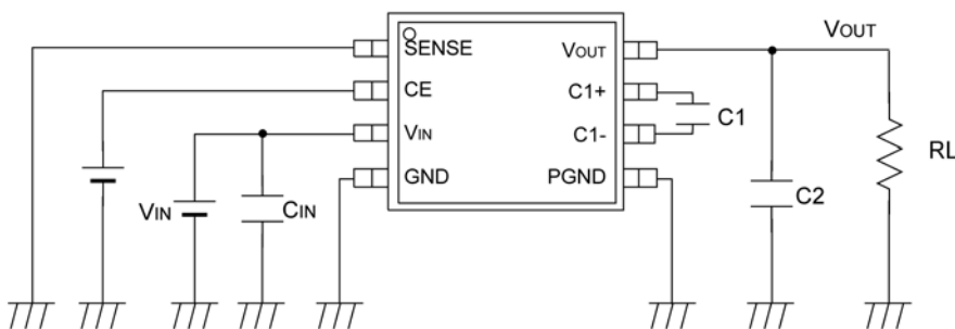
Doubler Output
