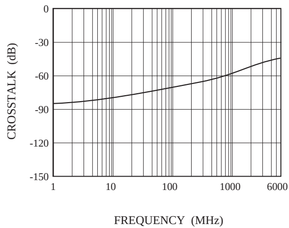
ANALOG CROSSTALK
