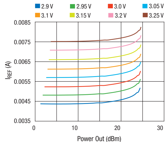
IREF vs. Power Out Across VREG
