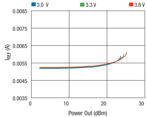
IREF vs. Power Out Across VCC
