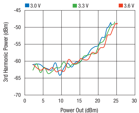
3rd Harmonic vs. Power Out Across V CC
