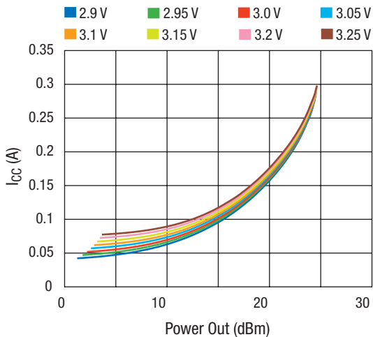
ICC vs. Power Out Across VREG
