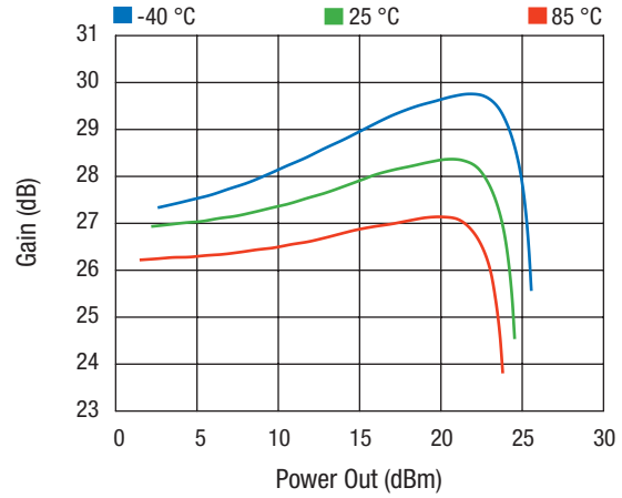
Gain vs. Power Out Across Temperature
