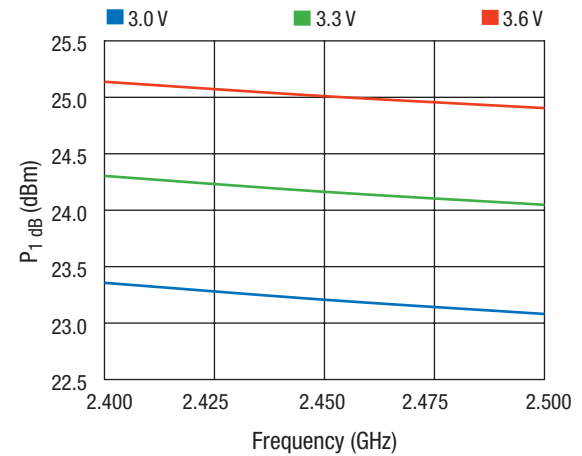
Output P 1 dB vs. Frequency Across V CC
