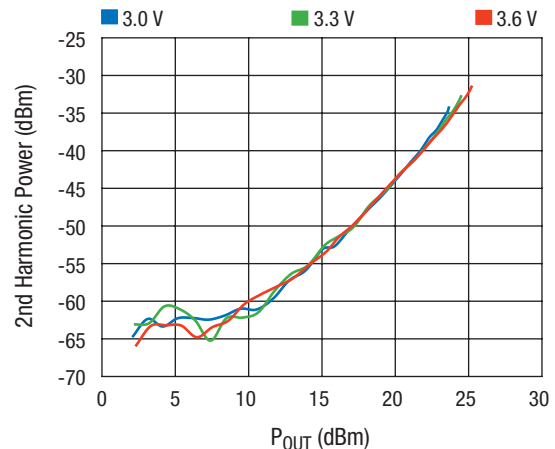
2nd Harmonic vs. Power Out Across V CC
