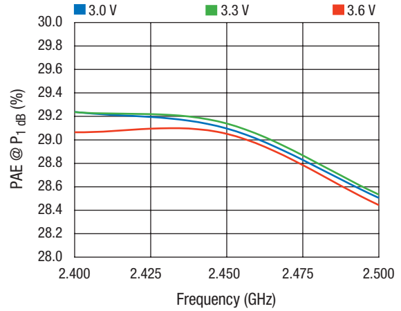
PAE @ P 1 dB vs. Frequency Across V CC
