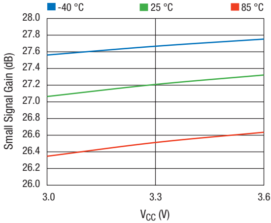
Small Signal Gain vs. V CC Across Temperature
