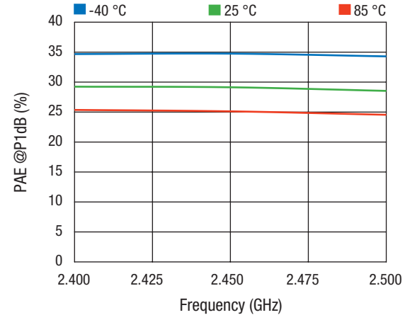
PAE @ P 1 dB vs. Frequency Across Temperature
