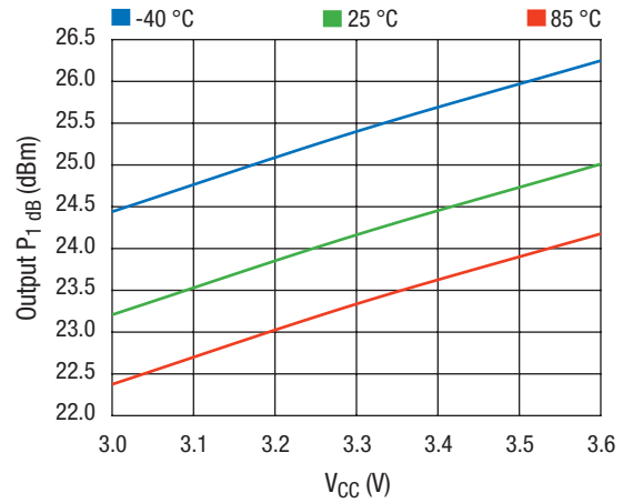
Output P 1 dB vs. V CC Across Temperature
