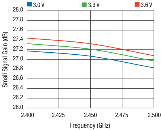
Small Signal Gain vs. Frequency Across V CC
