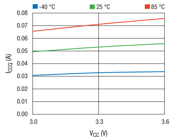
ICCC vs. V CC Across Temperature
