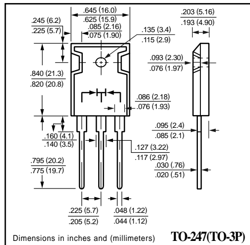
TO-247(TO-3P)
