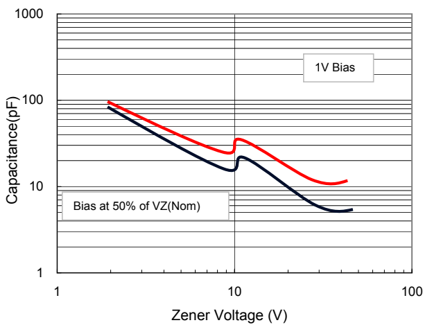
FIG 5 Typical Capacitance
