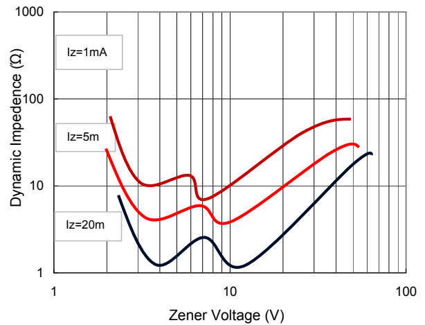
FIG 6 Effect of Zener Voltage on Impedance
