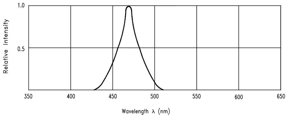
Fig.1 Relative Intensity vs. Peak Emission Wavelength
