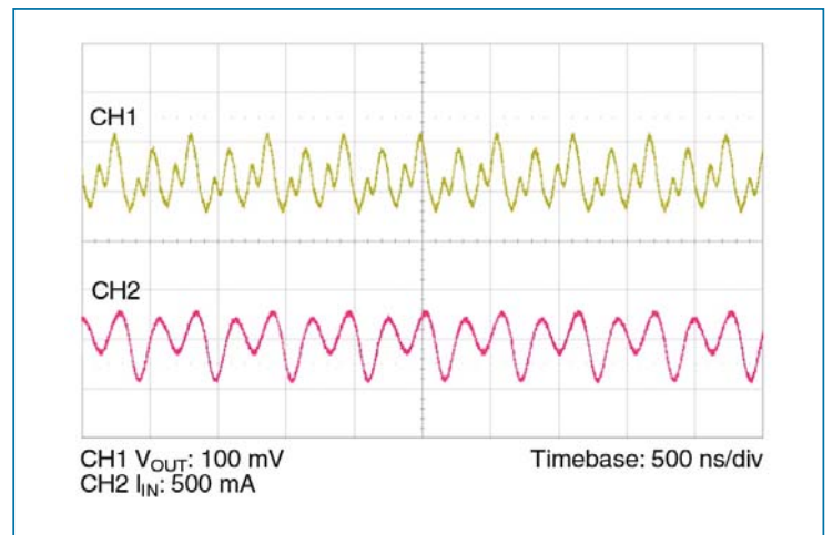
Figure 10 — Output voltage and input current ripple, 384 V_{IN} , 325 W no C_{OUT}
