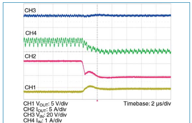
Figure 12 — Negative load transient (7.07 A – 0 A)
