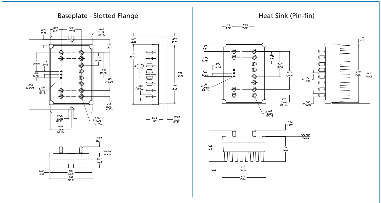
Figure 15 — Module outline
