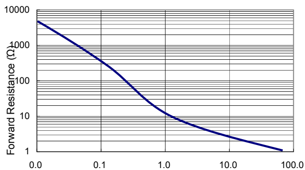
FIG 5 Forward Resistance vs. Forward Current
