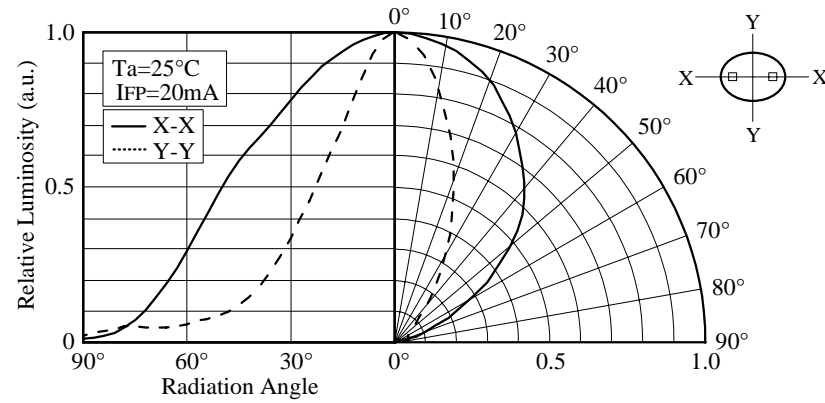
■ Directivity
