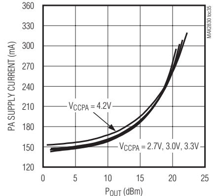
PA SUPPLY CURRENT vs. P_{OUT}
