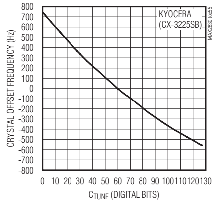
CRYSTAL-OSCILLATOR OFFSET FREQUENCY vs. CRYSTAL-OSCILLATOR TUNING BITS
