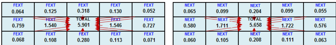
Figure 96 Single-ended cross-talk (in %) from simulations for port 15 and step input @ 120ps (20% to 80%) rise time and 2.625GHz BW
