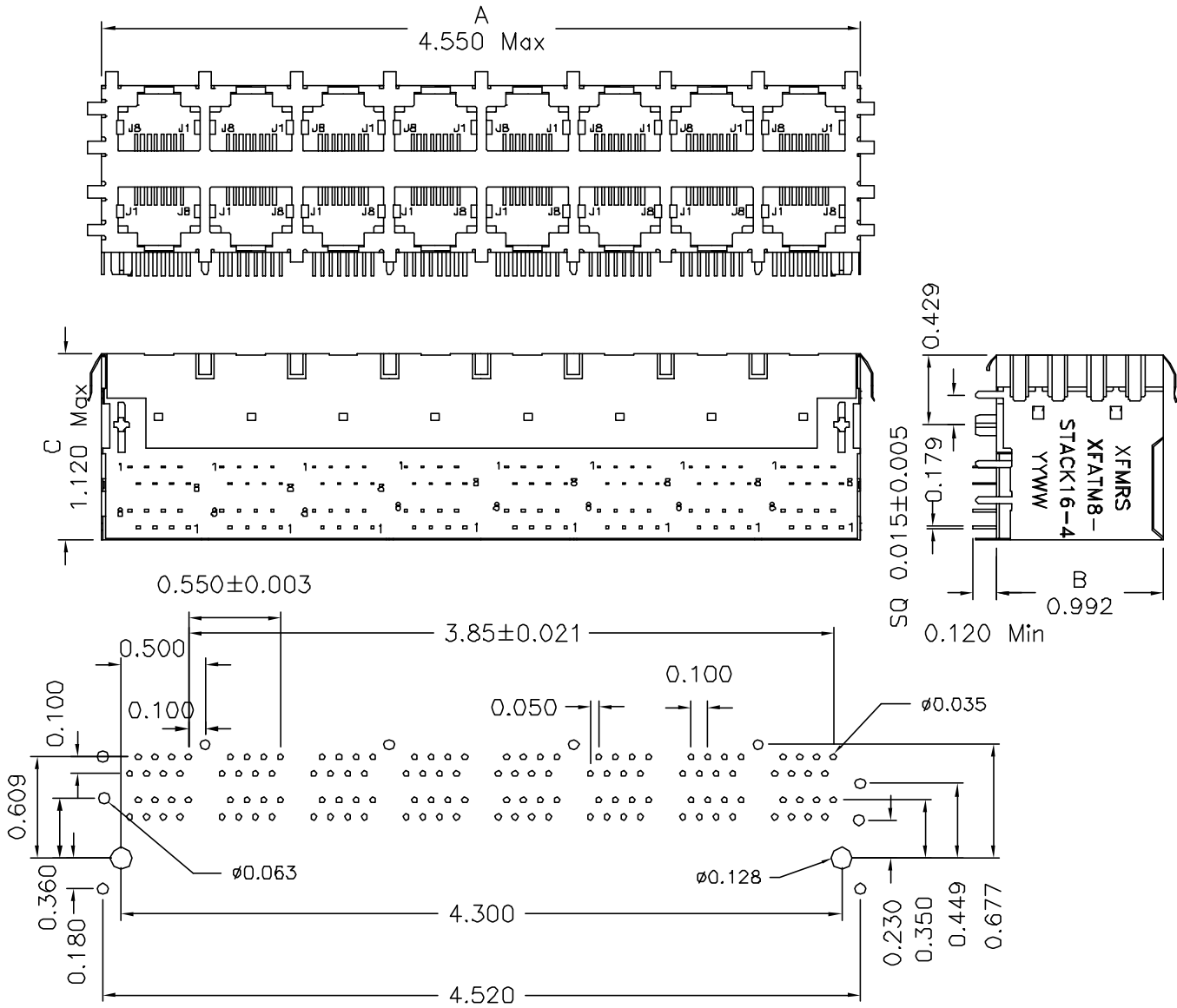
SUGGESTED MOUNTING PATTERN (COMPONENT SIDE)
